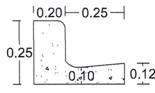
Detalle Conten
