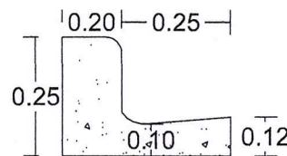
Detalle Conten
