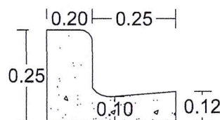
Detalle Conten
